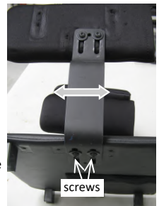
pic. 15.2: bracket adjustment
