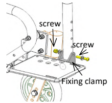
pic. 7.1: Height adjustment
