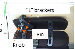
pic. 18: detachable mechanism
