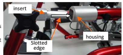
pic. 3.1: Inserting the legrest tube (detachable version)
