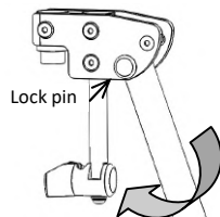
pic. 8.2: Elevating with spring pin knee angle adjustment
