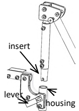
pic. 3.3: Inserting the legrest tube (vertical knee angle)
