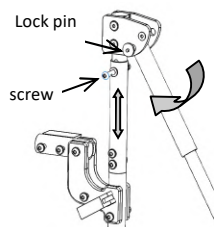
pic. 8.3: Vertical elevating and telescopic knee angle adjustment
