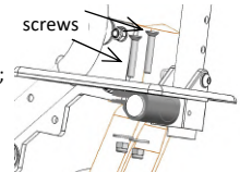
pic. 7.4: Angle adjustment
