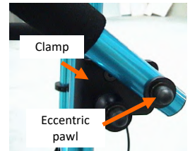
pic. 12: Tubular armrest
