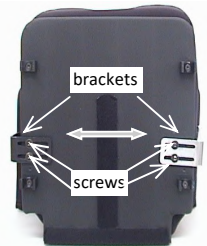
pic. 15.1: Seat width adjustment by the hip guides brackets
