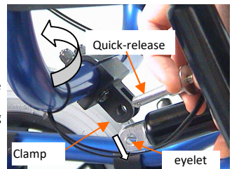
pic. 20: backrest tube installation
