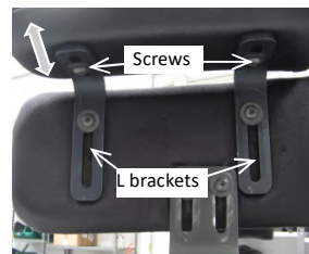
pic. 16.2: Width/depth adjustment
