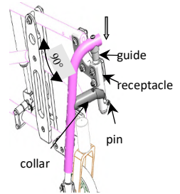
pic. 3.2: Inserting the legrest tube (swing-away version)
