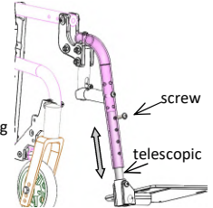
pic. 7.2: Height adjustment
